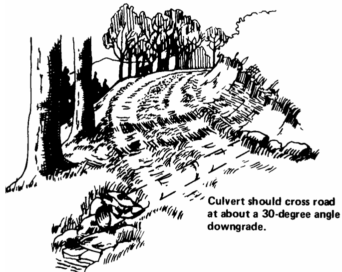
FIGURE 5 Culvert Placement
